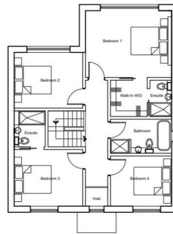
First Floor GIA 78m 2
